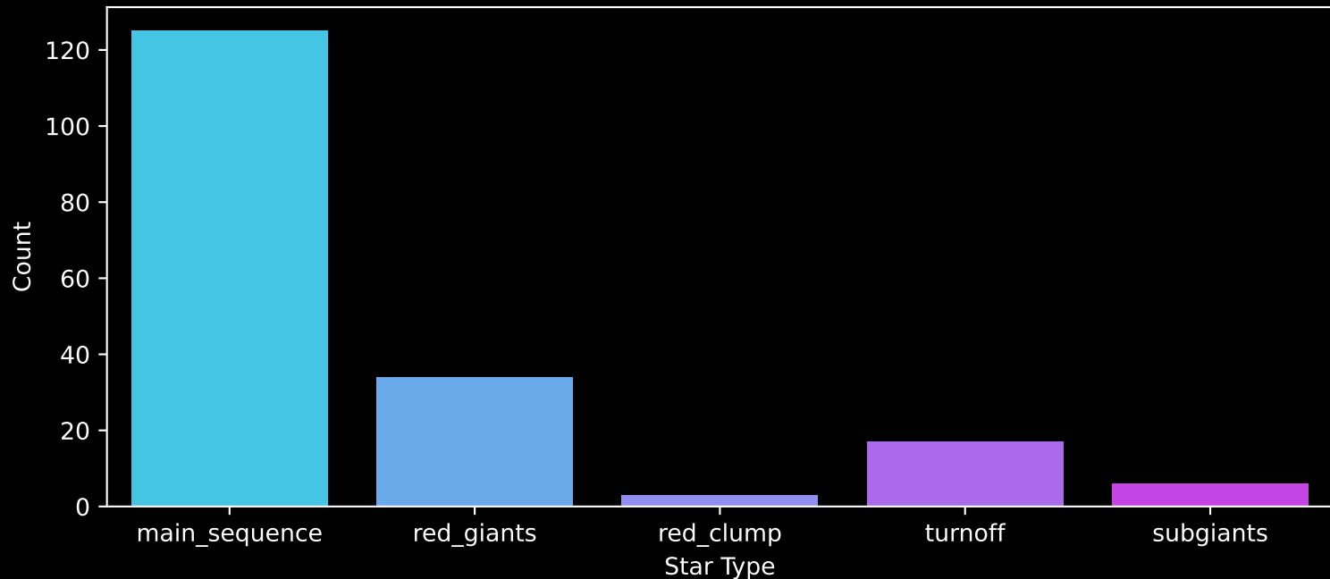
APOGEE DR17 Field: [150+60] Count plot of Star Type
