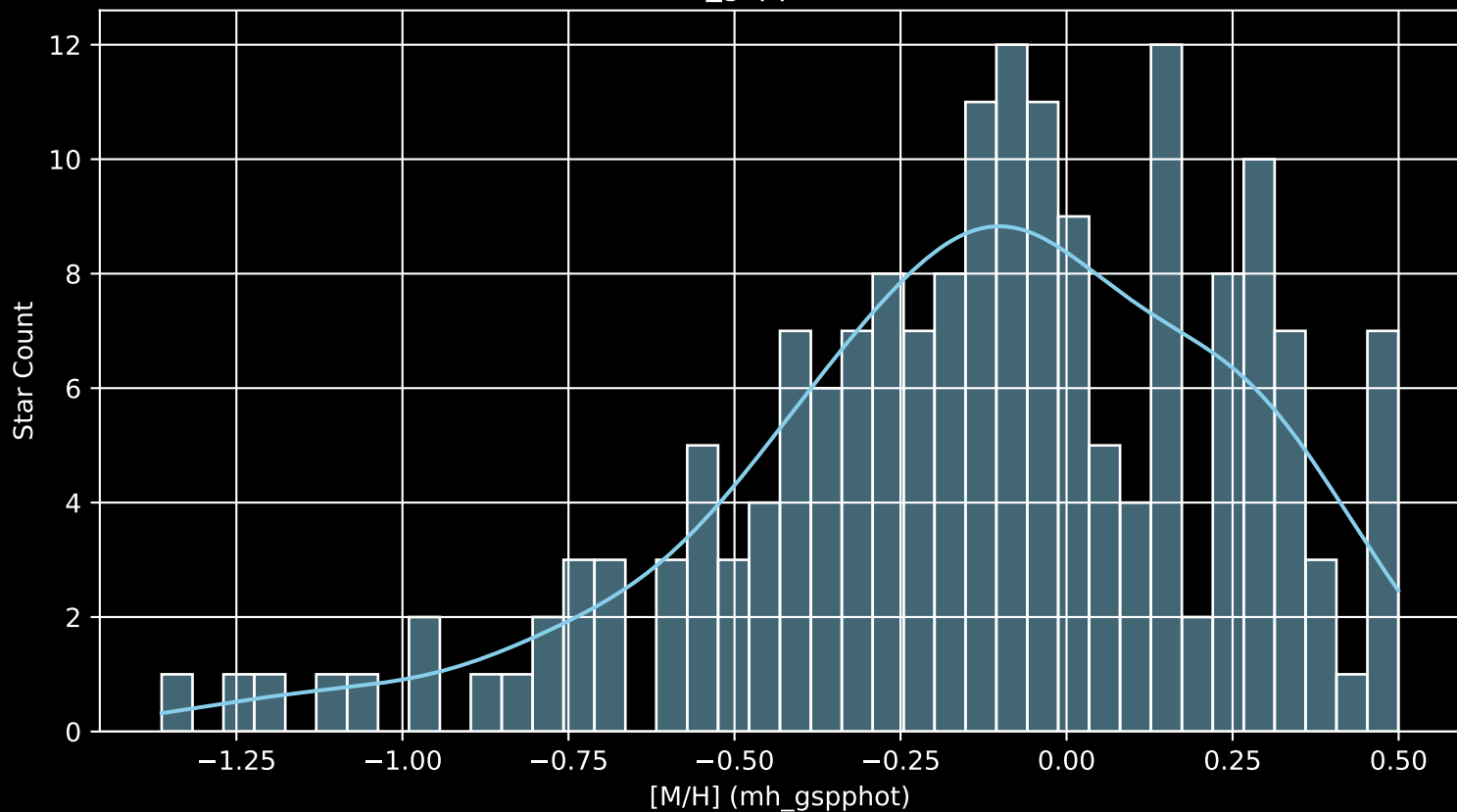
APOGEE DR17 Field: [150+60 [M/H] (mh_gspphot) (n= 177)
